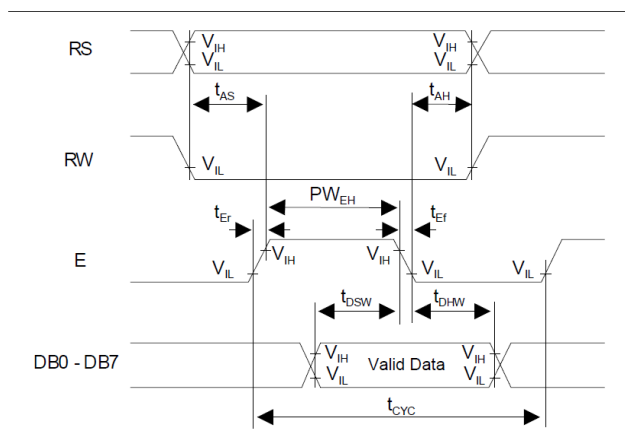
Fig.1 Write Operation Timing
